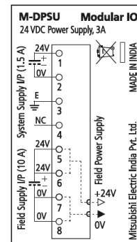
M-DPSU: Wiring description
