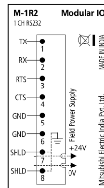
M-1R2: Wiring description
