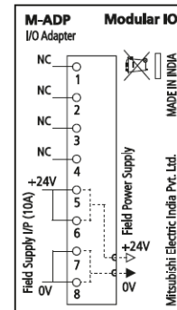
M-ADP: Wiring description
