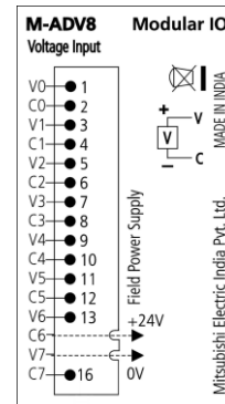
M-ADV8: Wiring description
