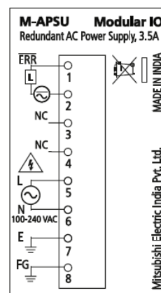
M-APSU: Wiring description
