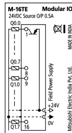
M-16TE: Wiring description
